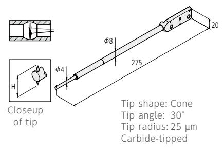
| Double-sided small hole arm stylus SPHW-33
